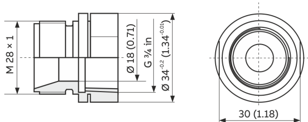
Screw connection G \frac{3}{4} in, simultaneous connection for Transair system 25 mm (pair)
