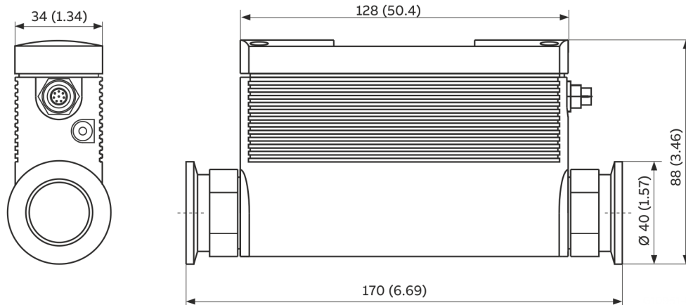
Figure 5: Flowmeter sensor FMT200-ECO2 with mounted small flange adapter
