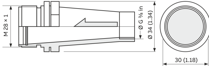
Screw connection G \frac{3}{8} in, connection for Legris hose adapter, pair) for inlet and outlet; inlet adapter with high-tech flow conditioner
