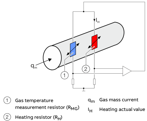
Figure 1: Analog measuring principle
