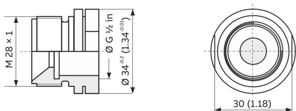
Screw connection G \frac{1}{2} in (pair) for inlet and outlet; inlet adapter with high-tech flow conditioner
