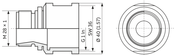
Screw connection G 1 in
