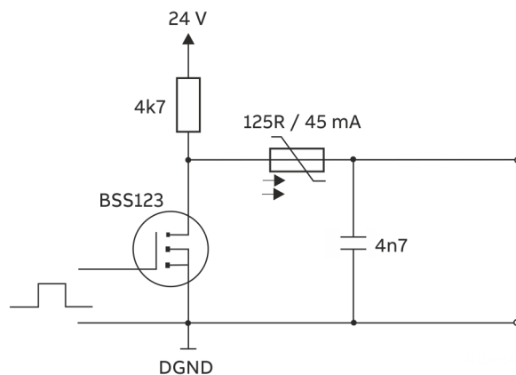
Figure 2: Digital output
