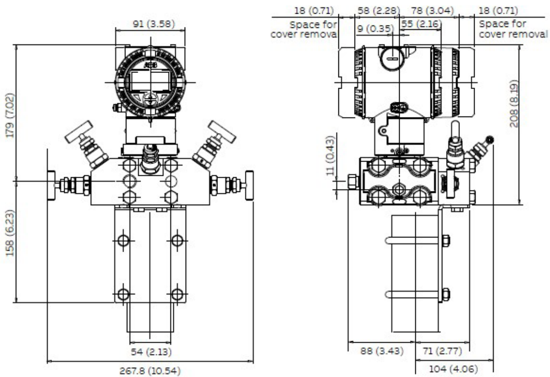
Differential pressure transmitter (266DSH, 266MSH) on manifold bracket with M26.D.A.V.5.V. (1/2 in. - 14 NPT female threaded inlet and flanged outlet according to IEC 61518/B)
