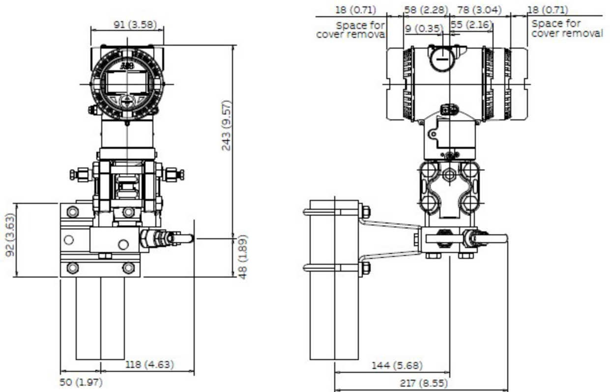
Pressure transmitter DP-Style (266PSH, 266VSH, 266RSx) with vertical flanges on manifold bracket with M26.D.A.V.2.V. (1/2 in. - 14 NPT female threaded inlet and flanged outlet according to IEC 61518/B)
