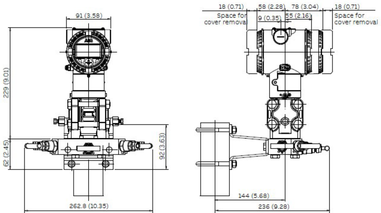
Differential pressure transmitter (266DSH, 266MSH) on manifold bracket with M26.D.A.V.5.V. (1/2 in. - 14 NPT female threaded inlet and flanged outlet according to IEC 61518/B)
