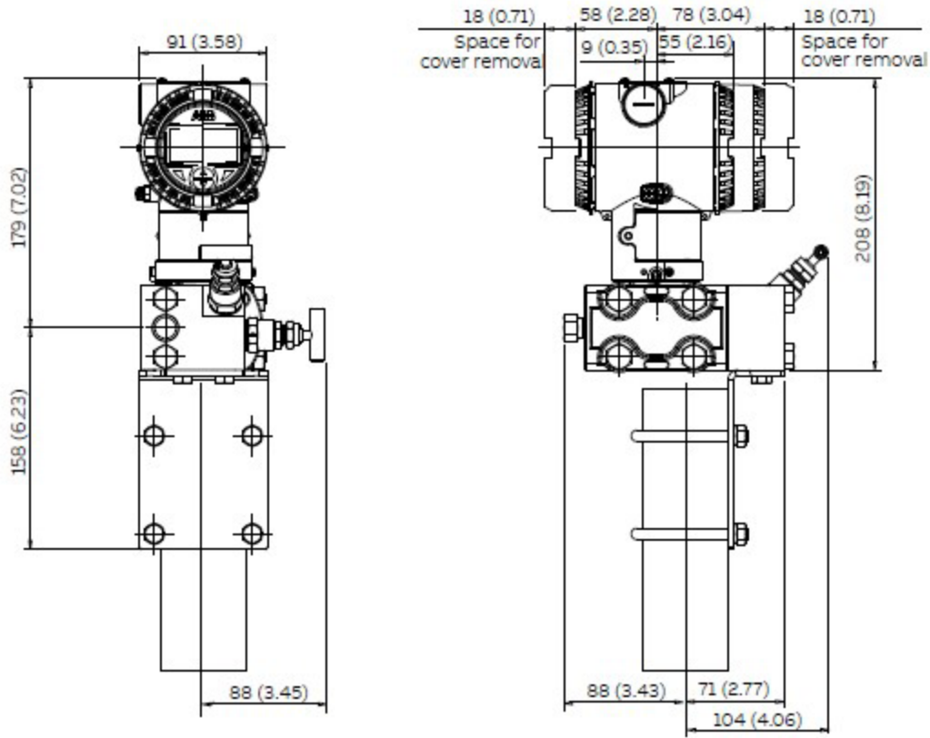
Pressure transmitter DP-Style (266PSH, 266VSH, 266RSx) with vertical flanges on manifold bracket with M26.D.A.V.2.V. (1/2 in. - 14 NPT female threaded inlet and flanged outlet according to IEC 61518/B)
