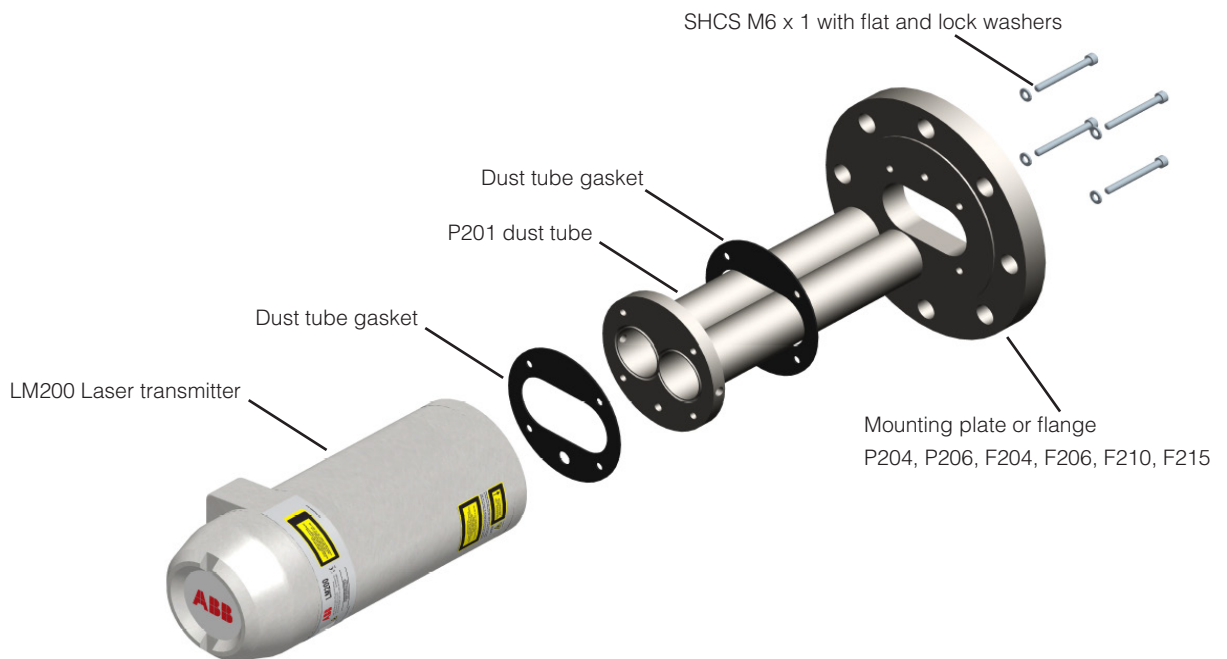
Figure 4 Mounting accessories
