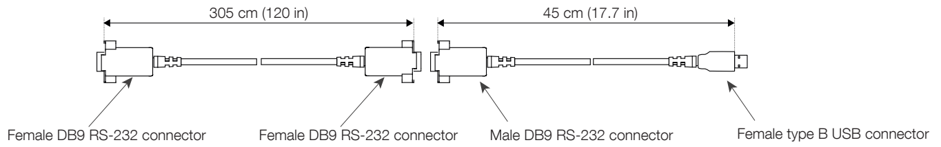
Figure 13 RS232 to USB cable (USBR)
