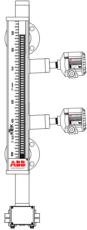
KM26 with side mounted insertion type switches
