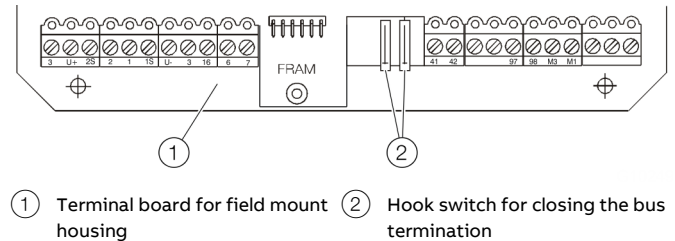
Figure 43: Bus termination
