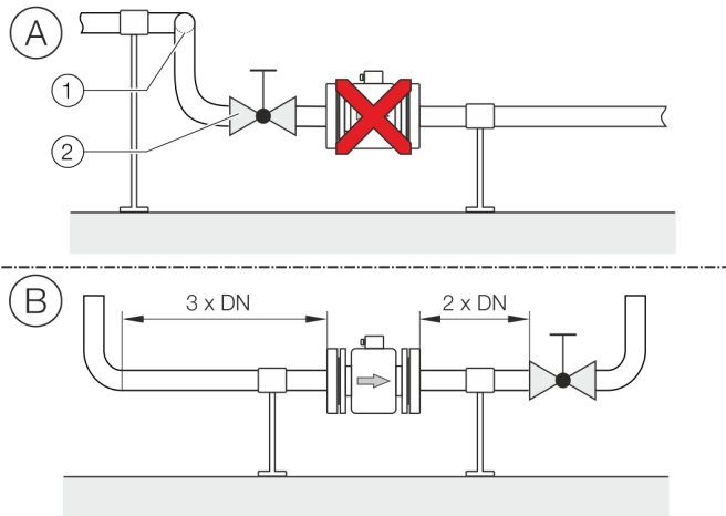
Figure 4: Inlet and outlet section, turn-off devices
