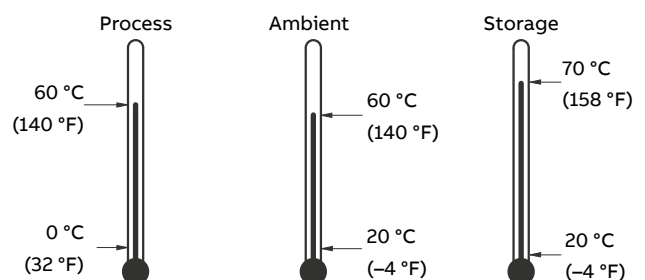
Figure 9 Temperature ranges
