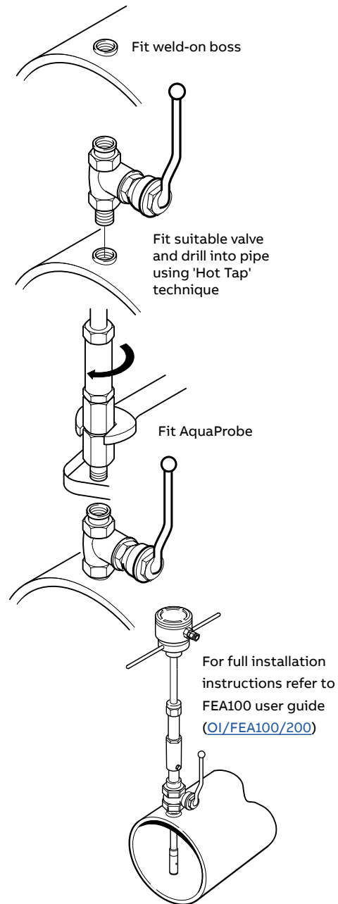
Figure 7 Typical installation (metal pipe)
