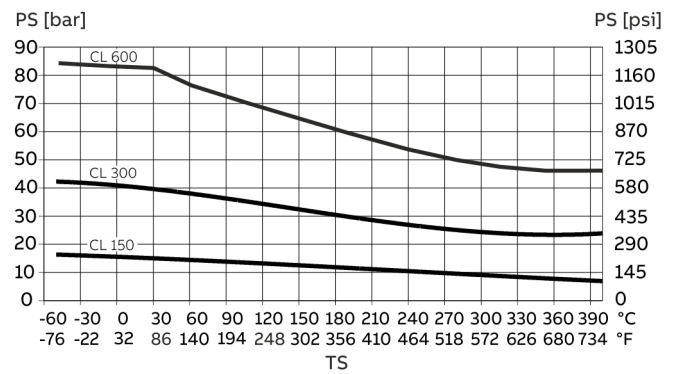
Figure 13: ASME flange made from stainless steel
