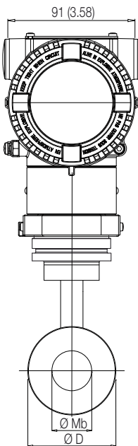
266HDH / 266NDH with barrel housing and direct mount seal S26JN in-line
