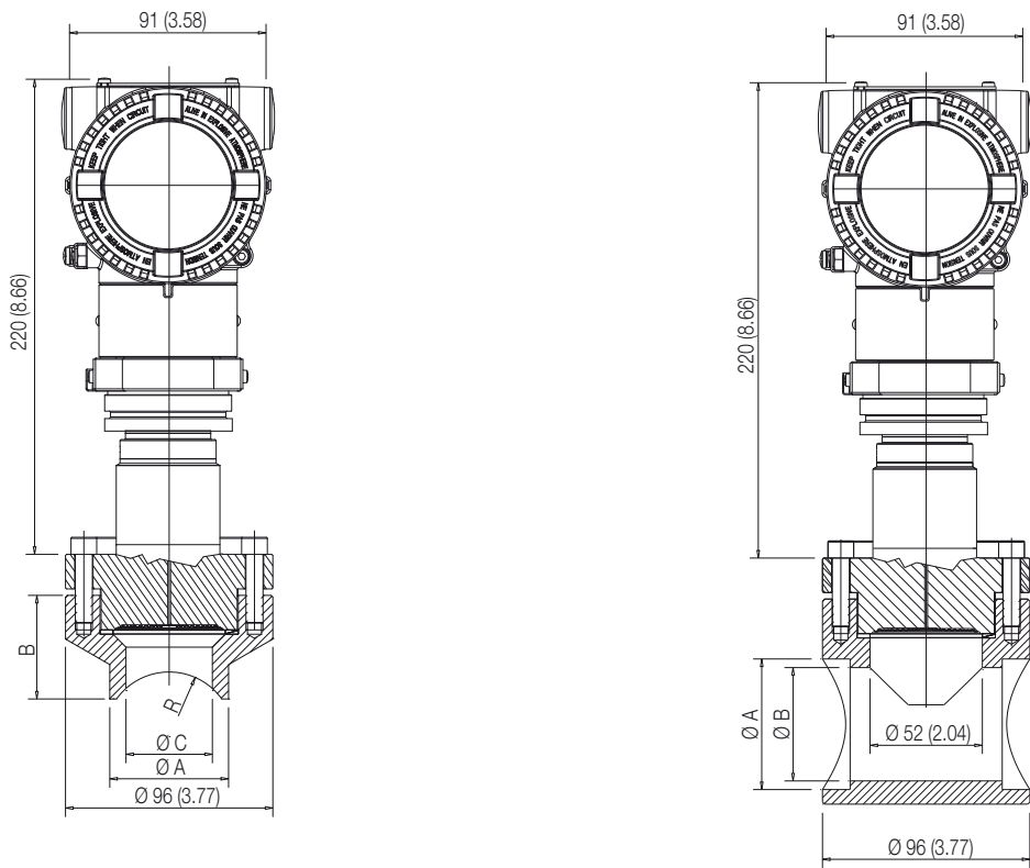
266HDH / 266NDH with barrel housing and direct mount seal S26VN saddle and socket
