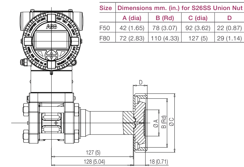
266DDH with barrel housing and direct mount seal S26SS Union Nut
