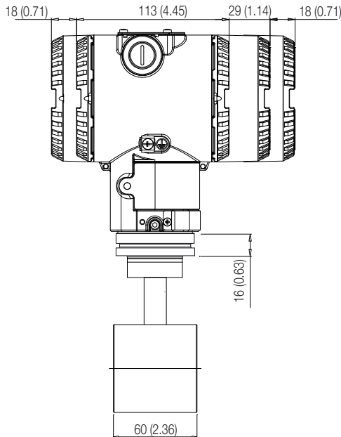
266HDH / 266NDH with barrel housing and direct mount seal S26JN in-line
