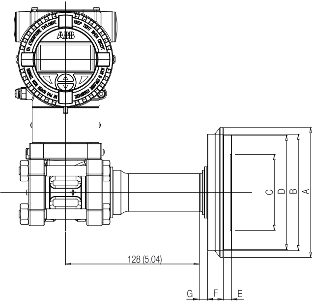
266DDH with barrel housing and direct mount seal S26SS Cherry Burrell
