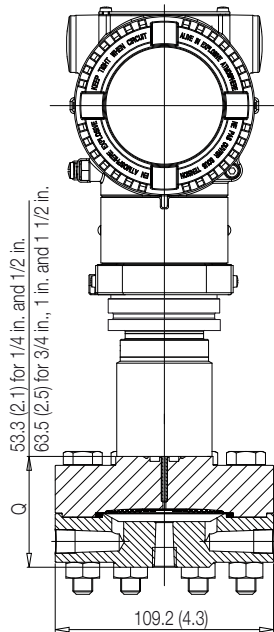
266HDH / 266NDH with barrel housing and direct mount seal S26TT off-line threaded flange
