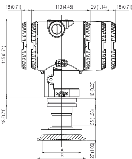
266HDH / 266NDH with barrel housing and direct mount seal S26SS Triclamp
