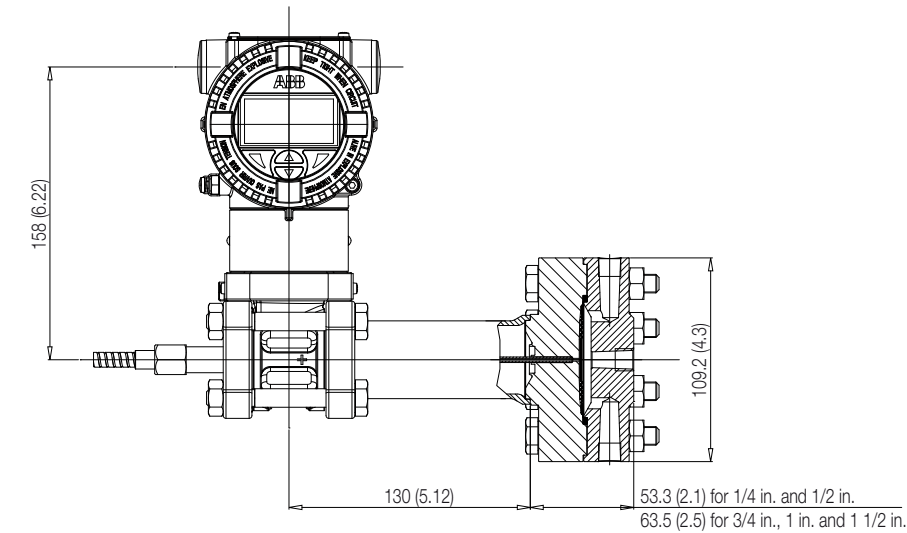
266DDH with barrel housing and direct mount seal S26TT off-line threaded flange
