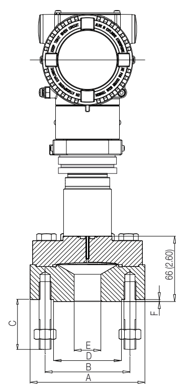
266HDH / 266NDH with barrel housing and direct mount seal S26Mx off-line flanged
