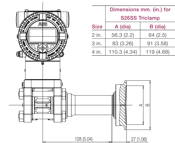
266DDH with barrel housing and direct mount seal S26SS Triclamp
