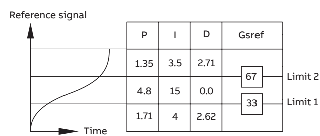
Figure 6 Gain scheduling example
