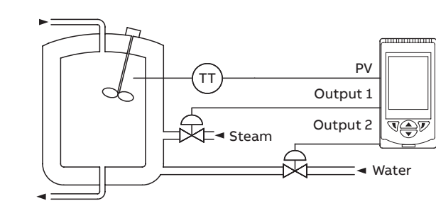
Figure 7 Split output control example
