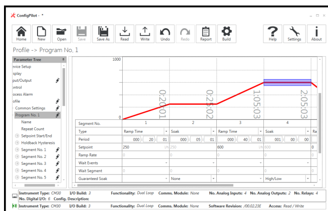
Figure 13 Profile configuration
