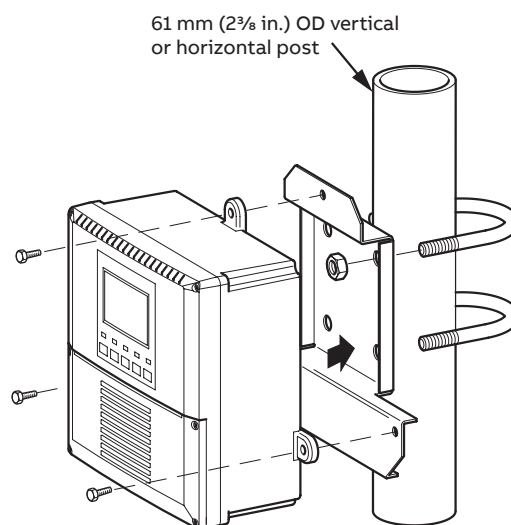
Pipe-mount detail
