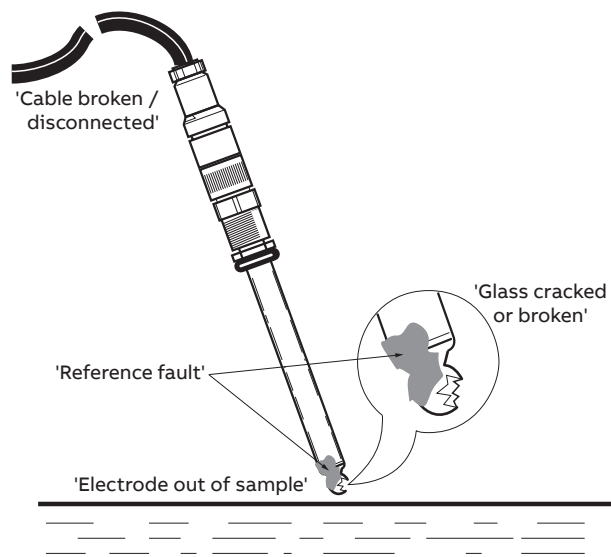
Just-in-time maintenance.
