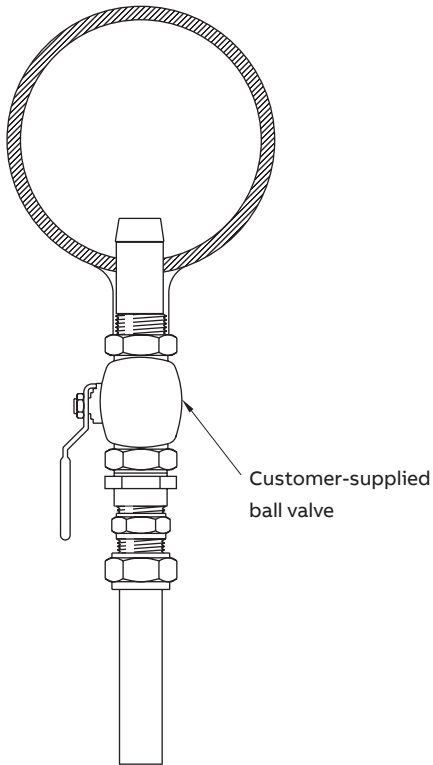
AP304 Hot-tap sensor – typical installation
