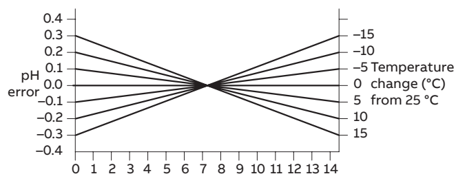
Temperature compensation
