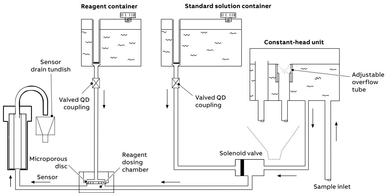
Figure 2 Schematic flow diagram
