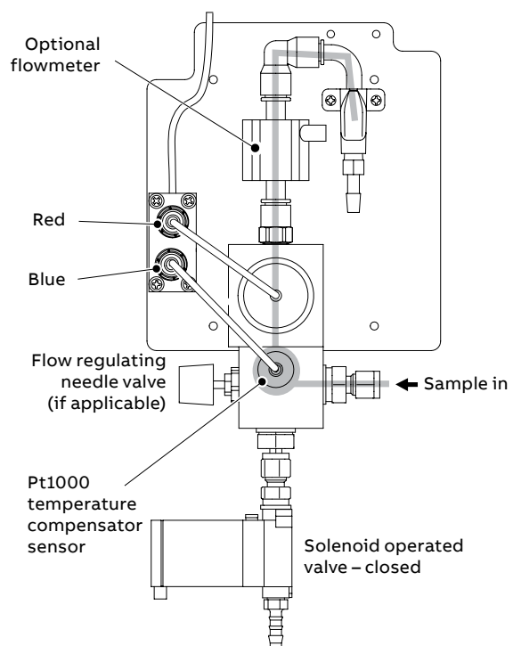
Flow during normal operation
