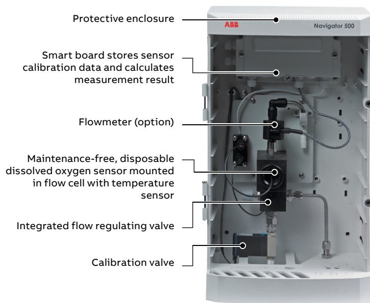
ADS550 wet section
