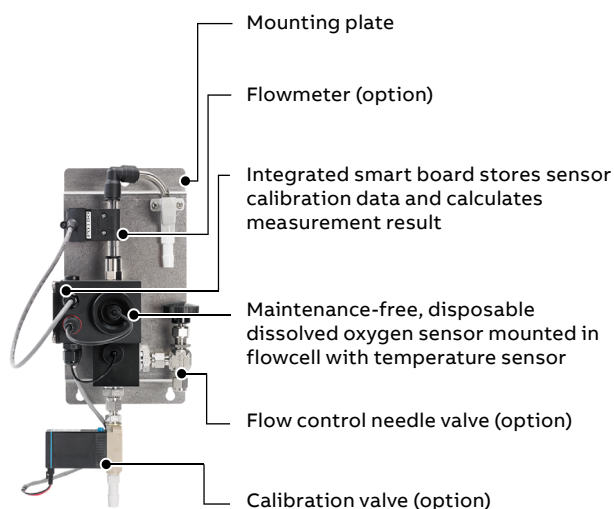
ADS551 wet section
