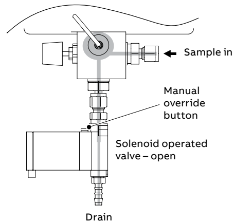
Flow during calibration or thermal overload condition
