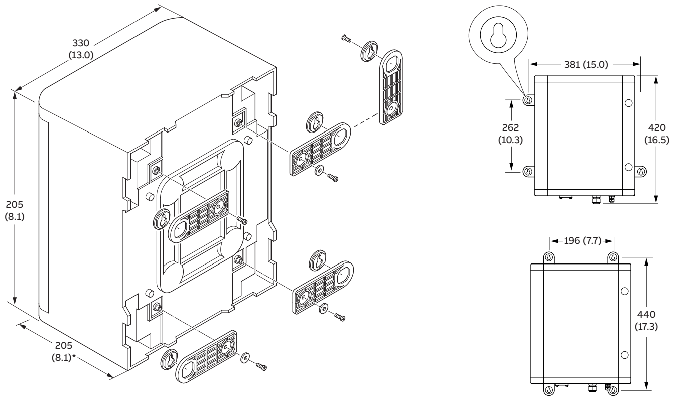
Fig. 15 Wall-mounting
