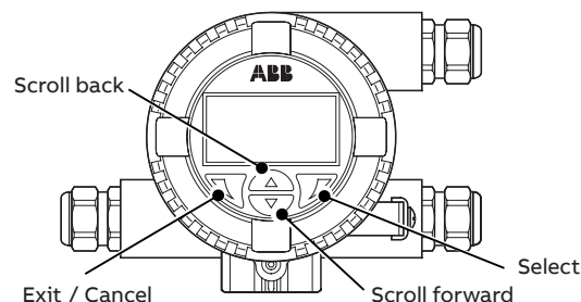
Figure 1 Navigation keys
