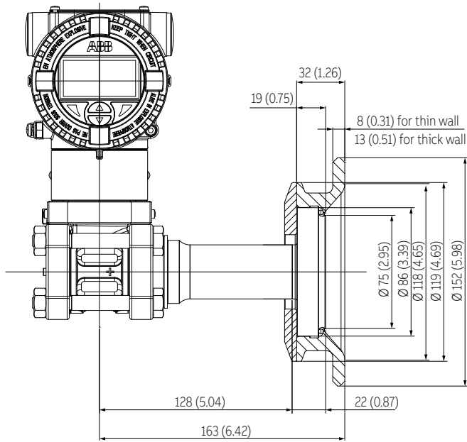
Figure 28 266DRH with barrel housing and direct mount seal S26SS Sanitary flush (For dimensions of S26 seals refer to the S26 datasheet)
