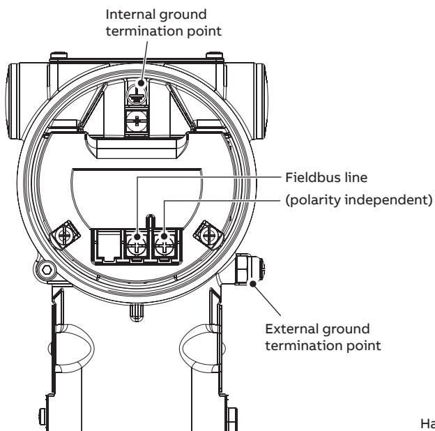
Figure 42 FIELDBUS Versions
