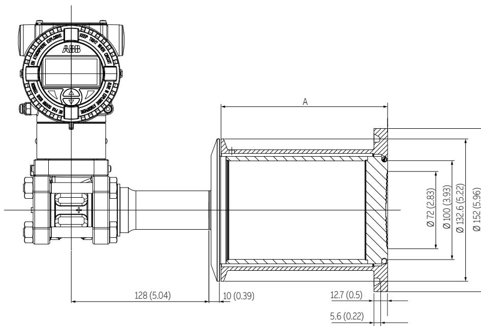
Figure 30 266DRH with barrel housing and direct mount seal S26SS Sanitary extended (For dimensions of S26 seals refer to the S26 datasheet)
