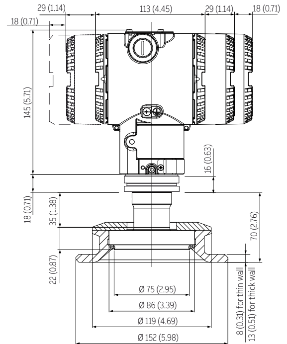
Figure 29 266HRH / 266NRH with barrel housing and direct mount seal S26SS Sanitary flush (For dimensions of S26 seals refer to the S26 datasheet)
