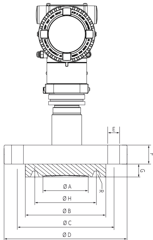
Figure 13 266HRH / 266NRH with barrel housing and direct mount seal S26RR flanged Ring Joint flush diaphragm (For dimensions of S26 seals refer to the S26 datasheet)
