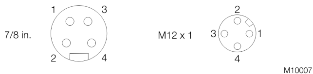
Fig. 7: plug connectors - fieldbus versions
