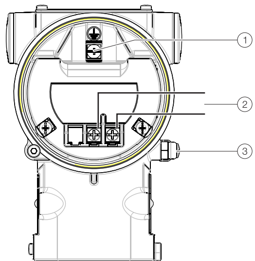
Fig. 8: Standard terminal block
